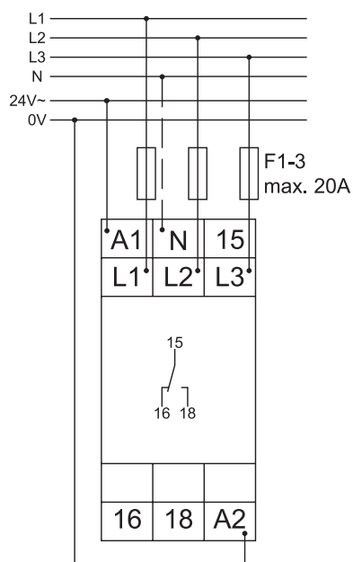
G2PM400VSY10 24V
